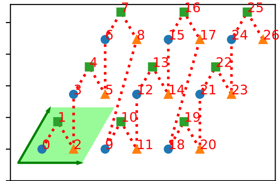
("grouped", [(0, 2, 1)], None)
