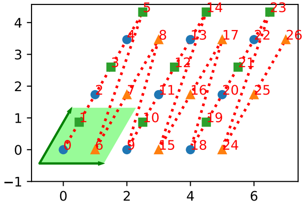
("grouped", [(0, 2), (1,)], None)
