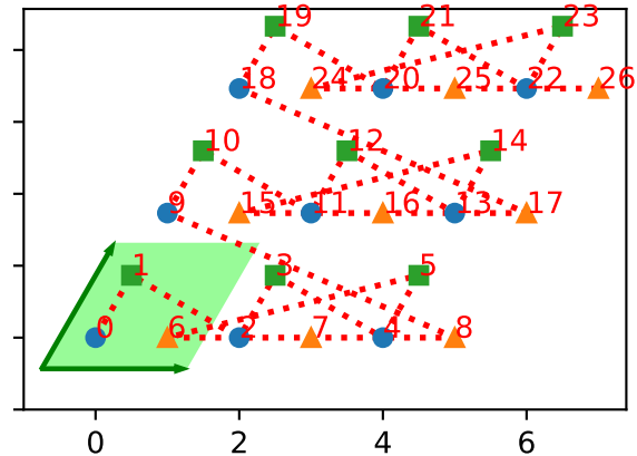
("grouped", [(0, 2), (1,)], [1, 0, 2])
