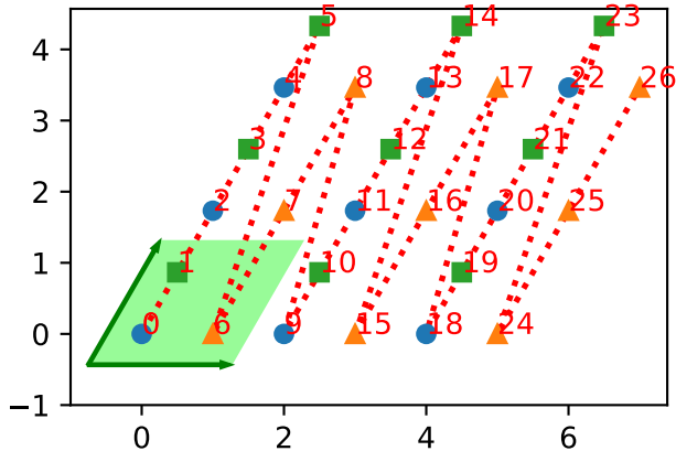
("grouped", [(0, 2), (1,)], None)
