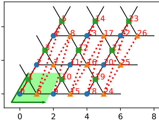
order='rings'
